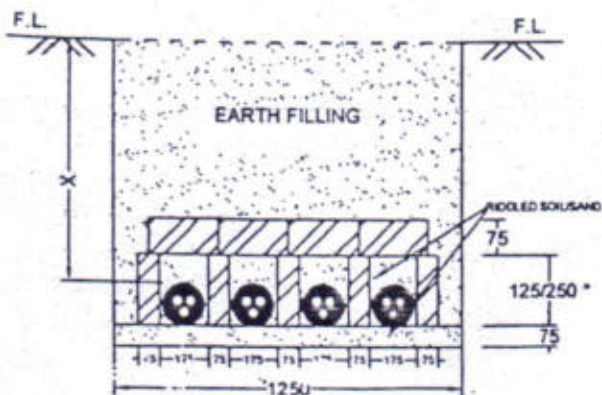
LAYING OF 4 NOS CABLES IN TRENCH
